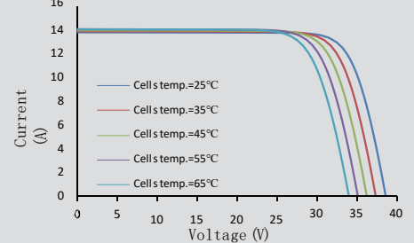
Current-Voltage (425W)
